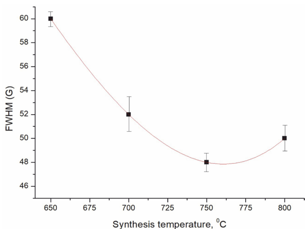
Fig. 2. Dependence of crystallinity of CNT samples on the temperature of synthesis.
