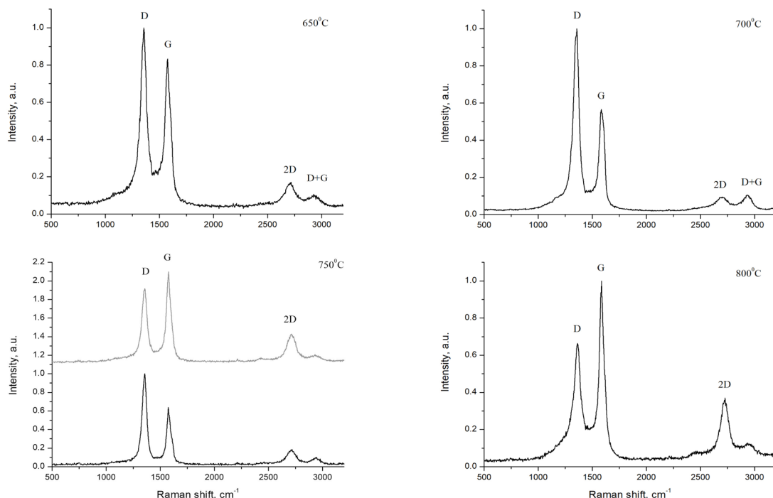
Fig.1. Raman spectra of MWCNTs synthesized on diatomite at different temperatures.
