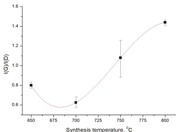
Fig. 3. The evolution of I(G)/I(D) ratio with the synthesis temperature.
