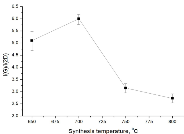
Fig. 4. Ratios of G and 2D Raman peaks intensity for different synthesis temperatures.
